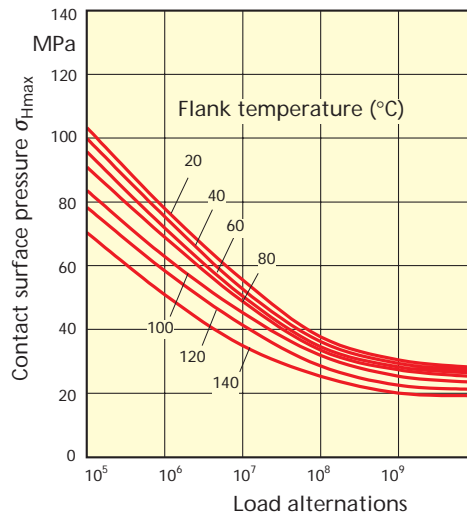
Diagram 12: Contact surface pressure \sigma_{Hmax} PA 6 G, grease lubrication
