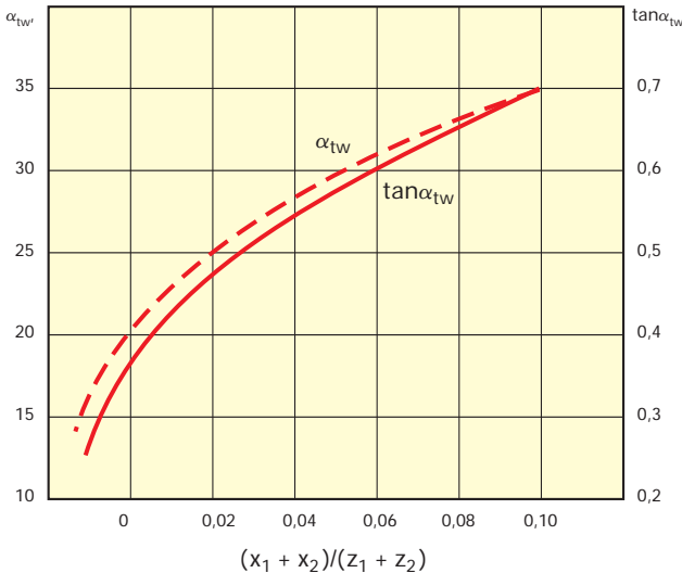
Diagram 4: Effective pressure angle \alpha_{tw} , \tan \alpha_{tw}
