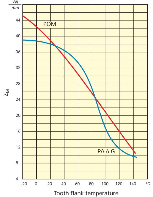
Diagram 8: Material factor for mating components K/St.
