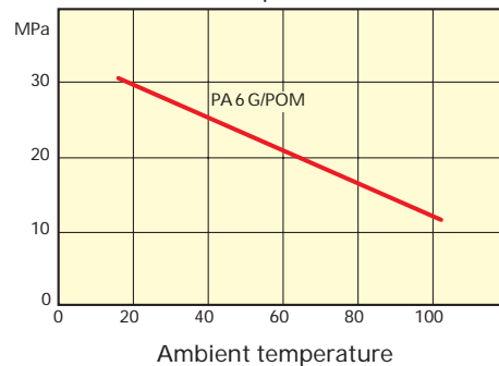
Diagram 1: Guiding value for permissible surface pressure
