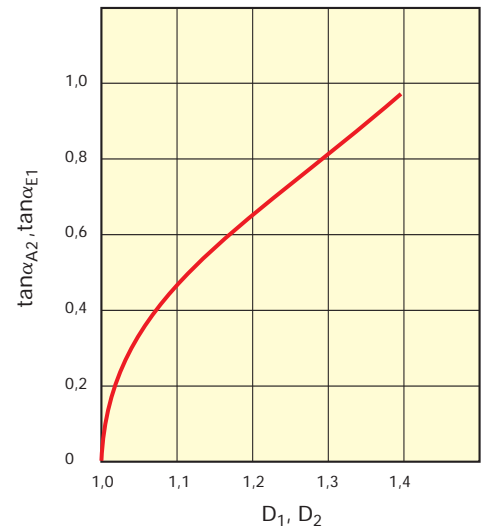
Diagram 5: Correction diagram for transverse contact ratio
