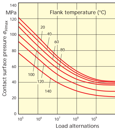
Diagram 13: Contact surface pressure \sigma_{Hmax} PA 6 G, oil lubrication
