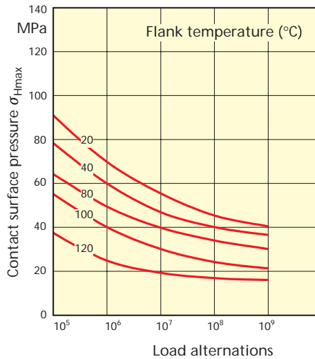
Diagram 14: Contact surface pressure \sigma_{Hmax} POM, dry running
