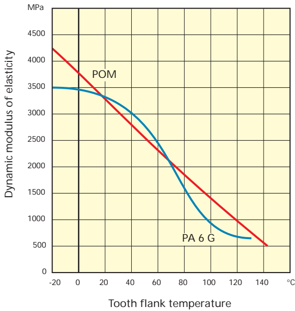
Diagram 7: Dynamic modulus of elasticity
