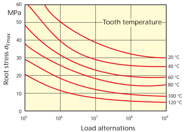
Diagram 10: Root strength of teeth \sigma_{Fmax} for PA 6 G
