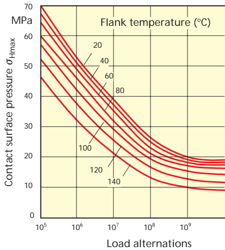
Diagram 11: Contact surface pressure \sigma_{Hmax} PA 6 G, dry running
